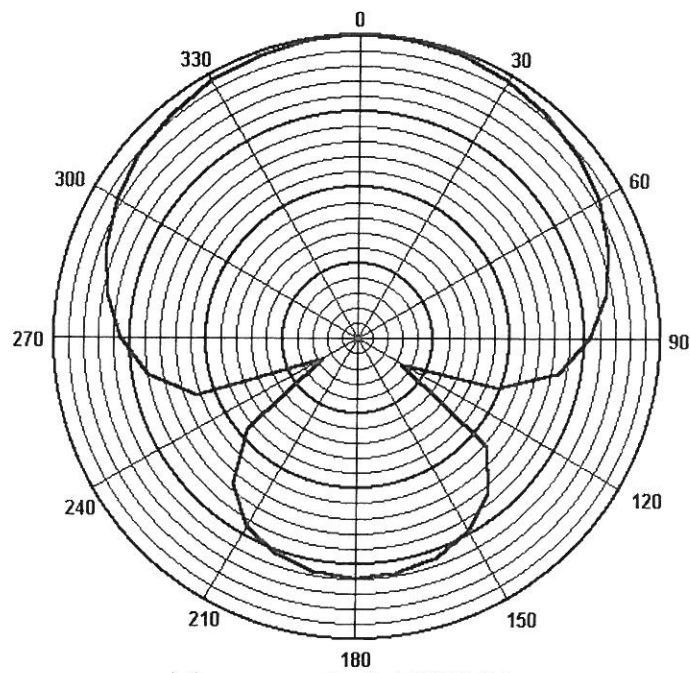
Figure 1: Polar pattern
