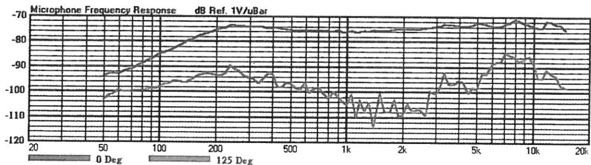
Figure 2: Frequency response
